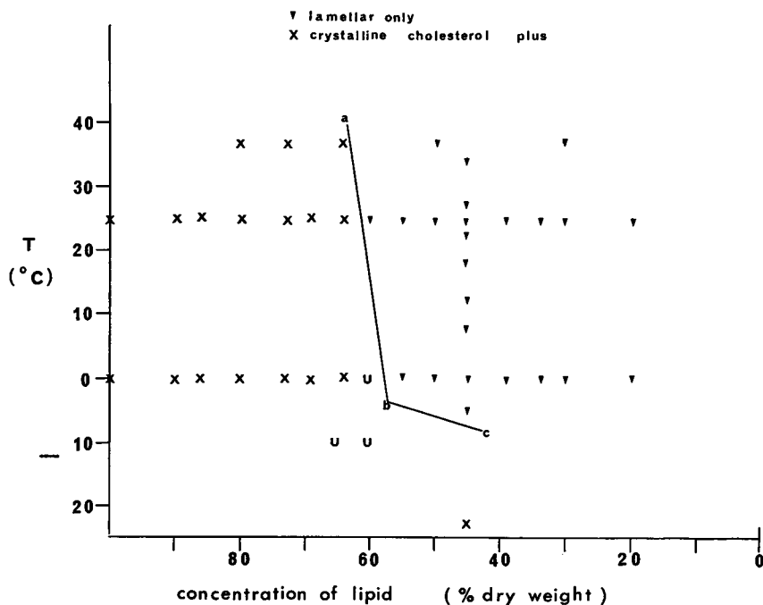
FIGURE 1 Phase Diagram. The marked points indicate region explored. X indicates crystalline cholesterol plus another phase. U indicates an unstable sample. ▼ indicates a single lamellar phase. The line abc depicts the boundary between the two major regions of the phase diagram.
